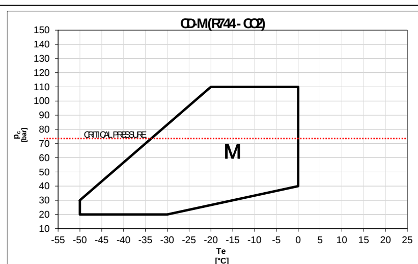
Fig. 4: CD0, CD200, CD2, CD4, CD400 - Limiti d'applicazione – Application limits – Champs d'application
